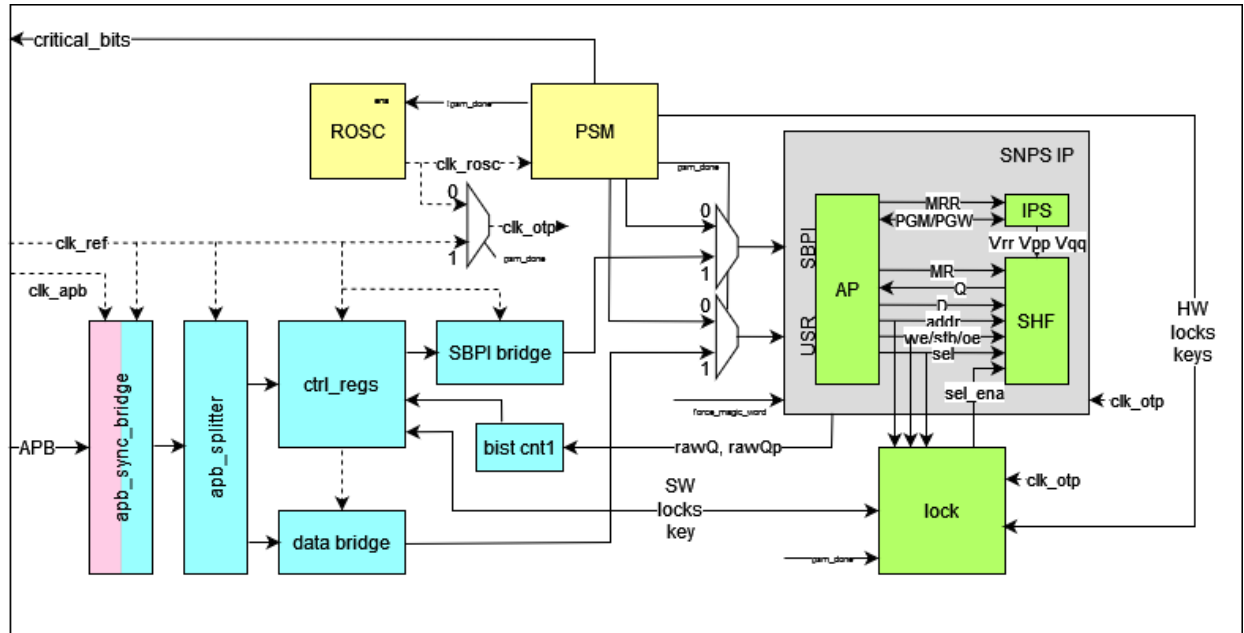
Figure 141. OTP architecture
