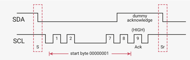
Figure 74. I2C Start Byte Transfer
