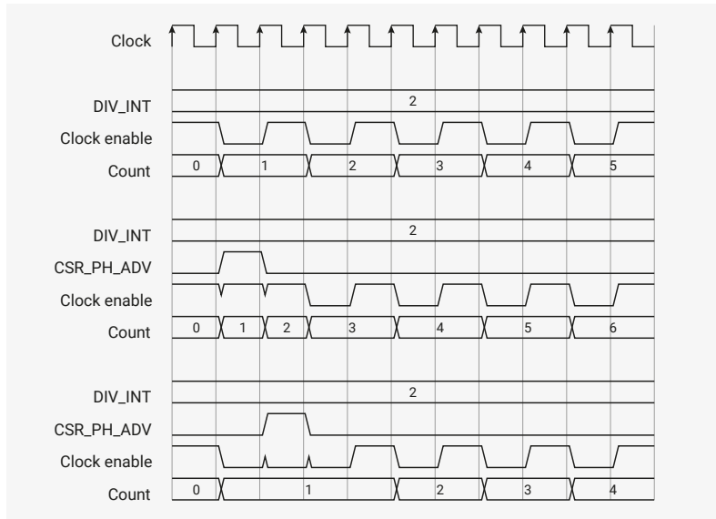
Figure 120. The clock enable signal, output by the clock divider, controls the rate of counting. Phase advance forces the clock enable high on cycles where it is low, causing the counter to jump forward by one count. Phase retard forces the clock enable low when it would be high, holding the counter back by one count.
