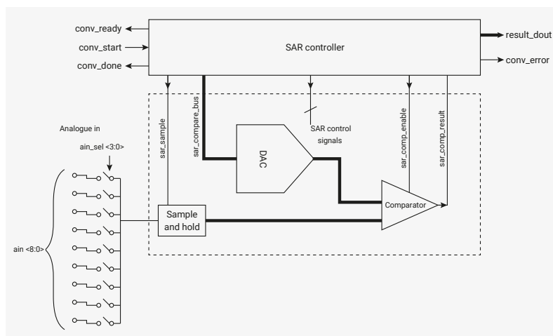
Figure 109. SAR ADC Block diagram QFN-80
