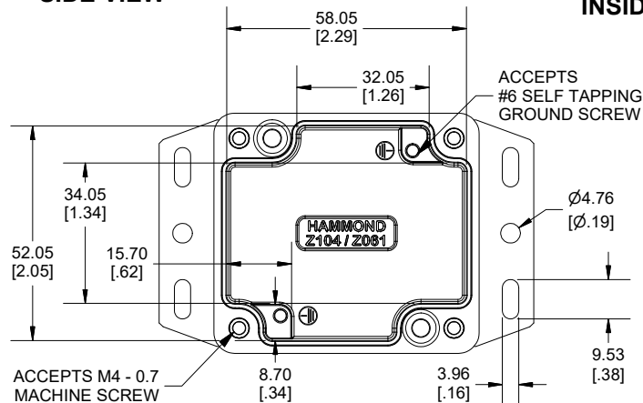
INSIDE BOX
