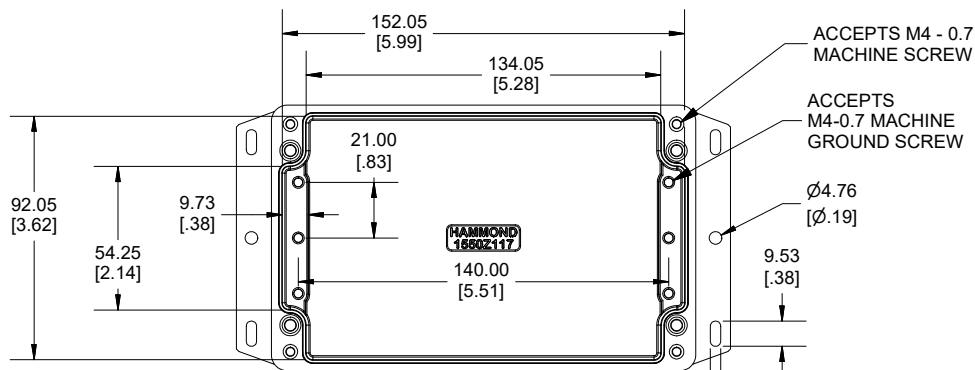
INSIDE BOX
