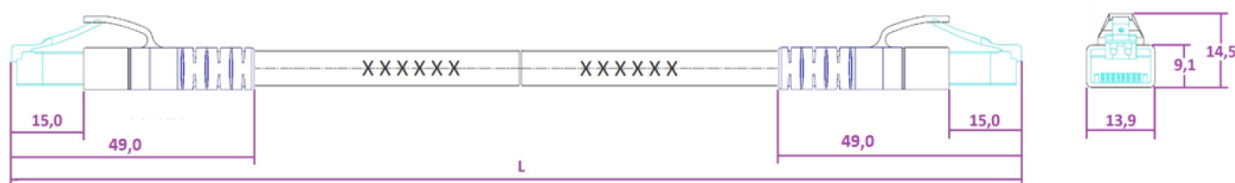
Dimensional drawing
