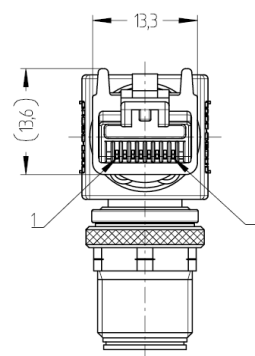
Jack RJ45
