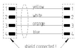
Contact Configuration
