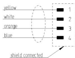
Contact Configuration
