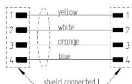
Contact Configuration
