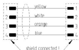
Contact Configuration
