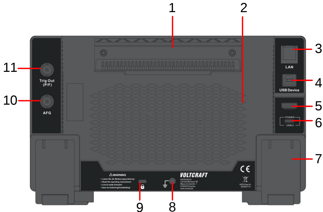
Figure 3-2: Rear Panel
