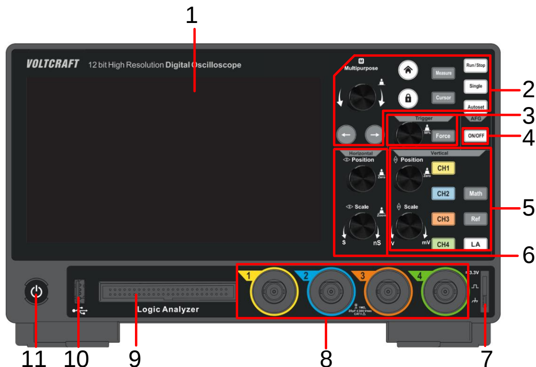
Figure 3-1: Front panel
