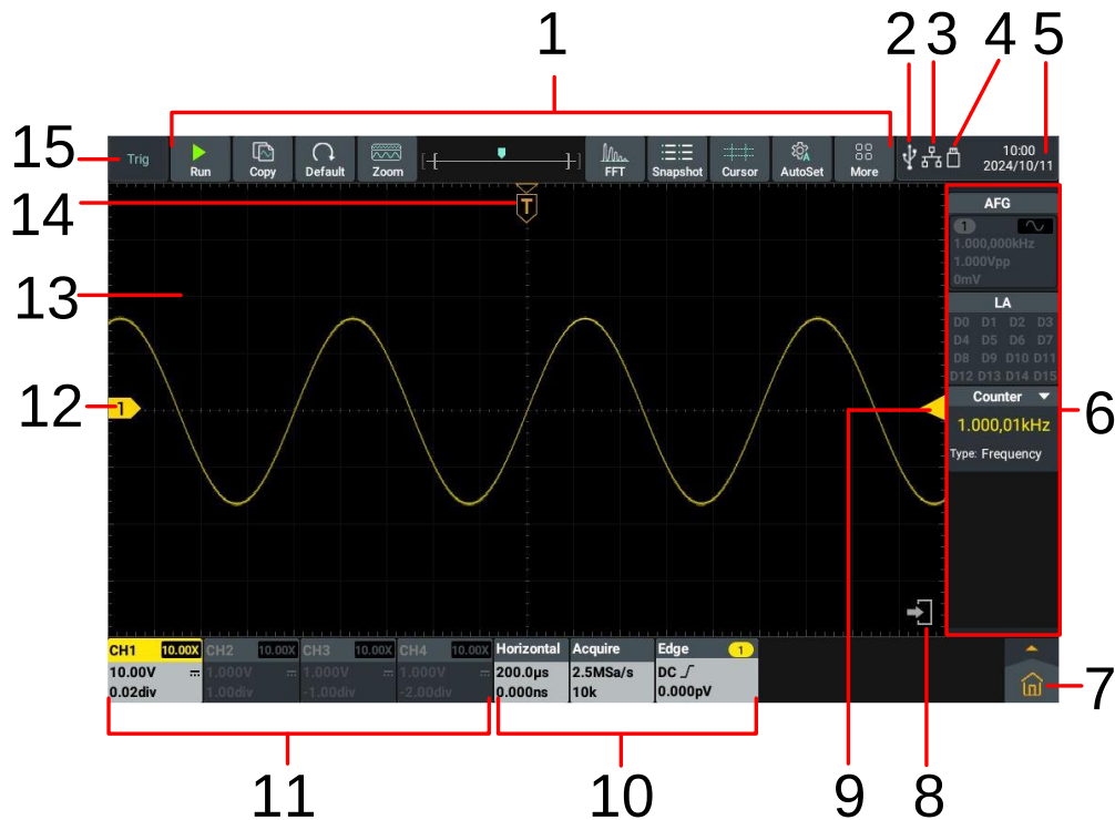
Figure 3-3: Illustrative Drawing of Display Interfaces
