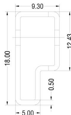
7Pin SIP Tube
