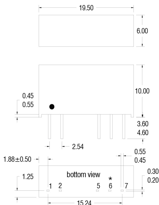
SIP Package
