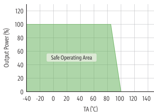
Temperature Derating
