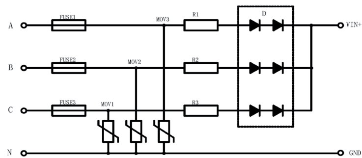
Photo 2: 4kVAC Differential Mode Surge High Requirements Recommended External Circuit - Half Wave Rectification
