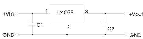
Positive output application circuit
