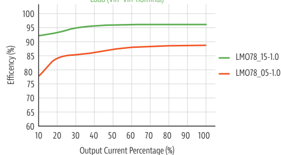
Positive Output Efficiency Vs Output Load (Vin=Vin-nominal)
