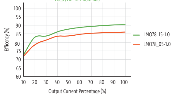
Negative Output Efficiency Vs Output Load (Vin=Vin-nominal)
