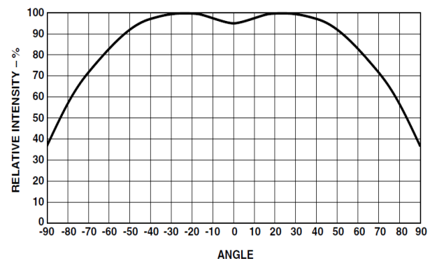
Figure 5: Radiation Pattern
