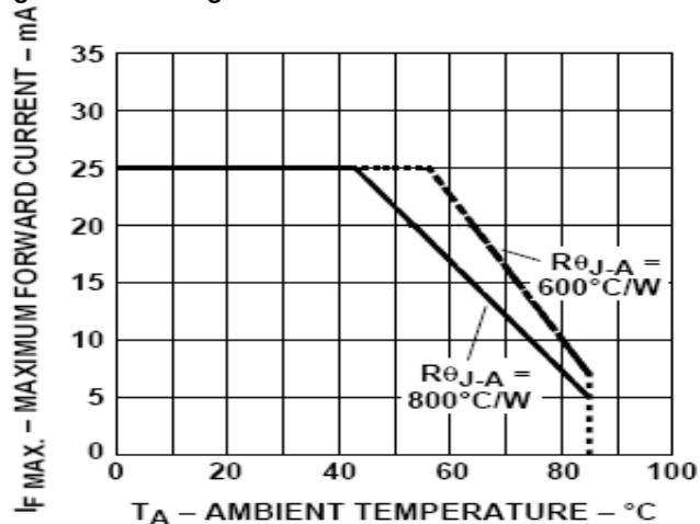
Figure 6: Derating Curve
