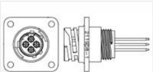
TE Part #1-788130-1 CPC RCPT,PSTD,SZ 11-4 LF
