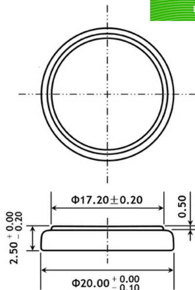
Dimension Drawing
