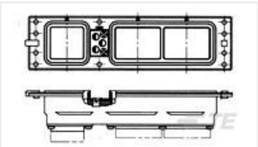
TE Part #2-211991-2 RECEPT ASSY,SZ 2,ARINC 600
