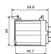
062.08 with relay
