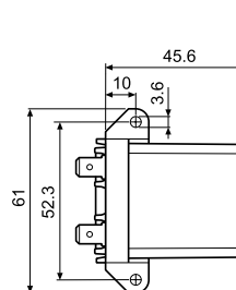
062.60 with relay
