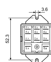
062.05 with relay
