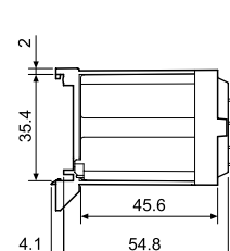
062.07 with relay
