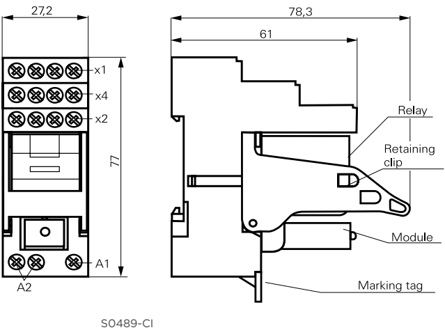
Package with PT78 722 / PT78 742
