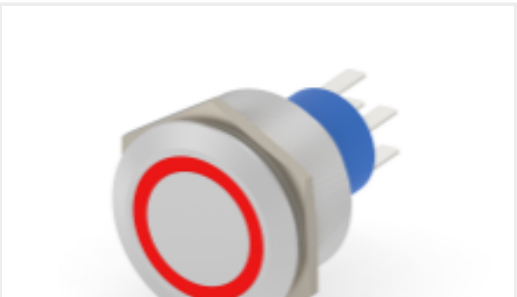
TE Part #3-2317656-3 AV25 DPL 3A MOVING RING RED 12V
