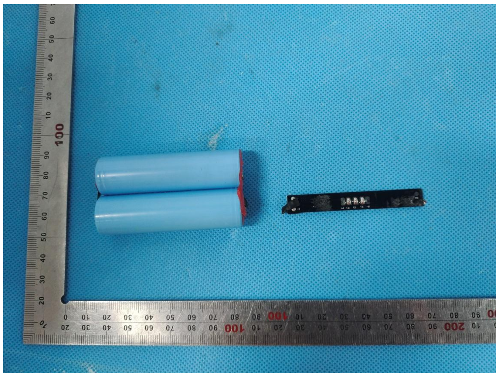
Fig. 14 – battery view
