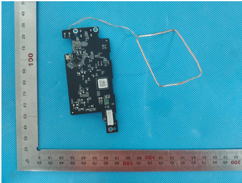
Fig.7 – PCB view
