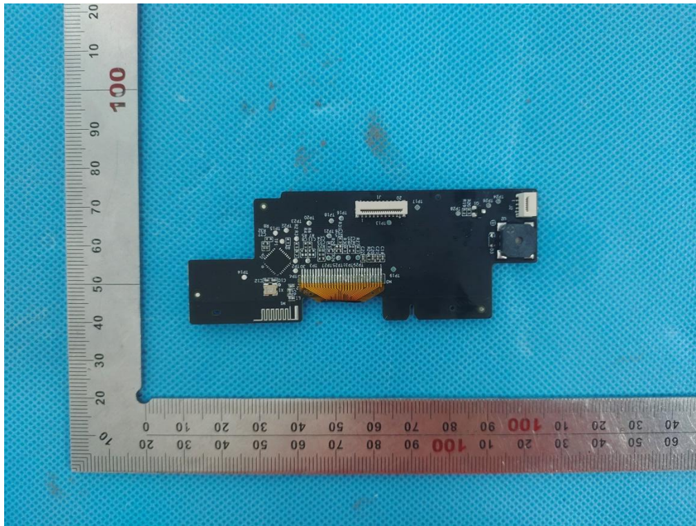
Fig. 9 – PCB view
