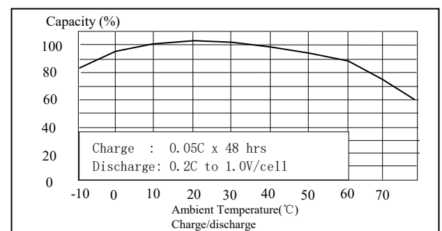
Charging Efficiency
