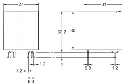
Relay Mounted on PCB (Reference Information)
