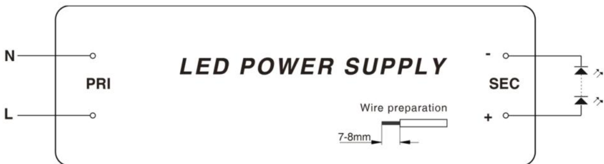
Wiring Diagram
