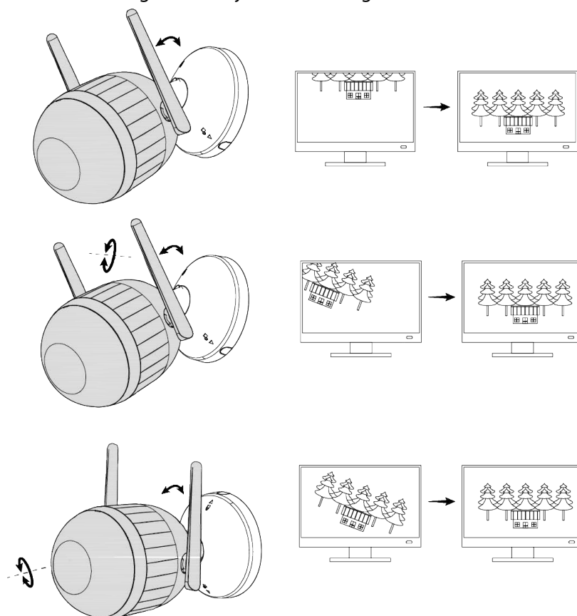
Figure 4-8 Adjust the lens angle
