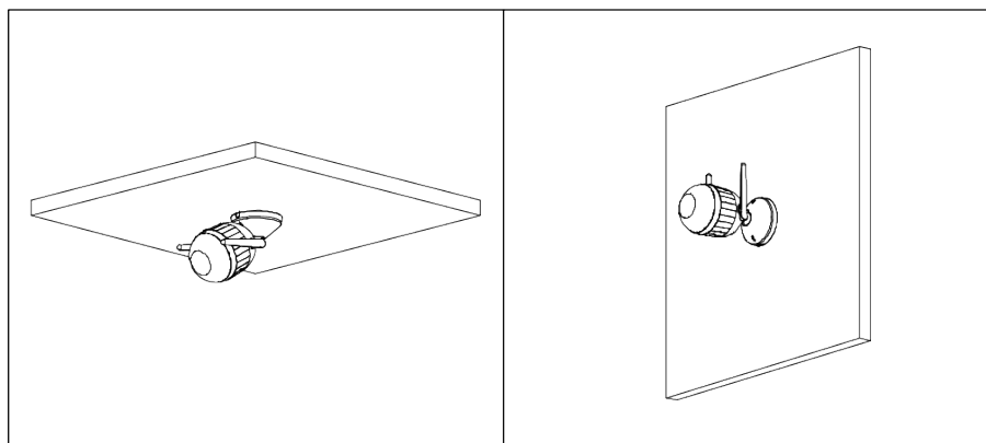
Figure 4-3 Installation methods
