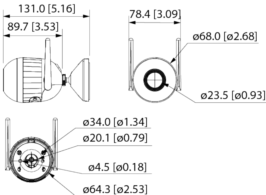
Figure 4-2 Dimensions (mm [inch])
