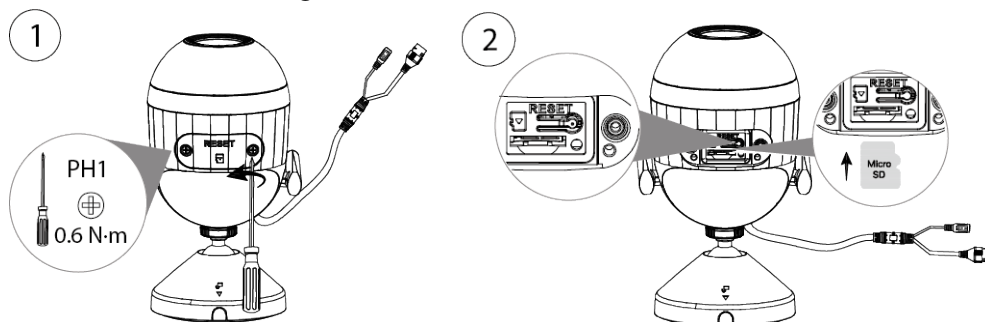
Figure 4-4 Install the SD card
