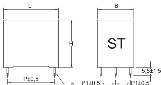
6 terminals execution
