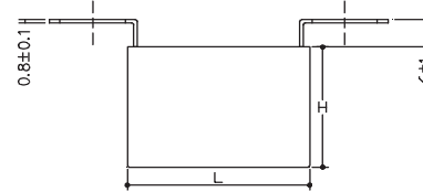
Fixing pitch and distance between lugs (mm)
