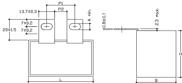
Style VN-VNM8 (for L=57,5mm only)
