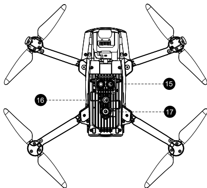
15 TOF assisted height determination system
