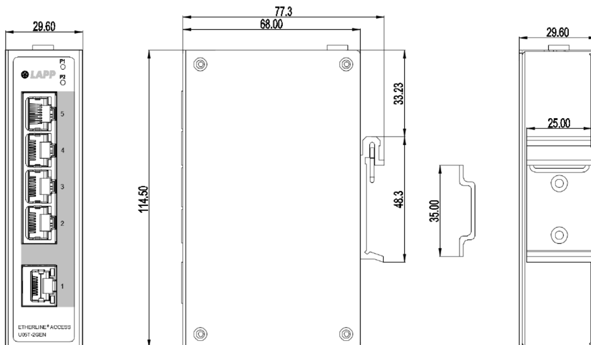
Dimensional drawing (U05T-2GEN)
