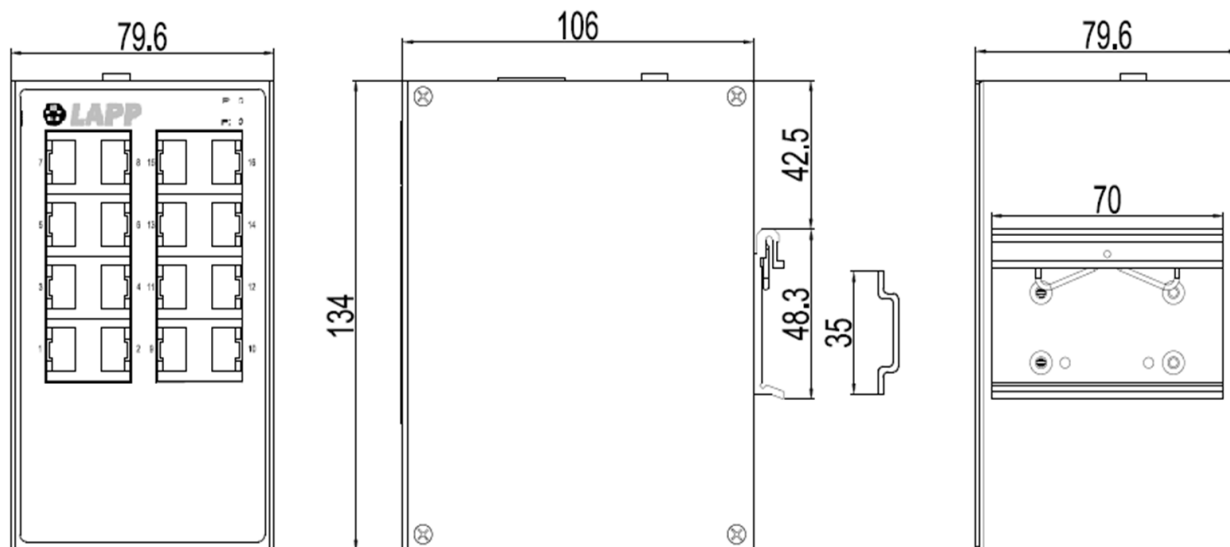
Dimensional drawing
