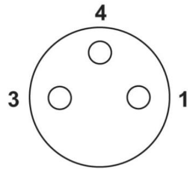
Pin assignment M8-jack, 3-pol, A-coded
