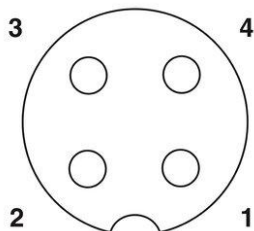
Pin assignment M12-jack, 4-pol, A-coding
