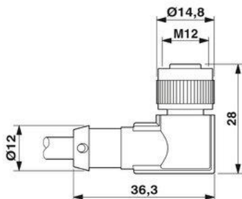
Jack M12 x 1, angled, with LEDs
