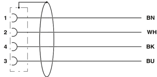
Pin assignment from M12-jack
