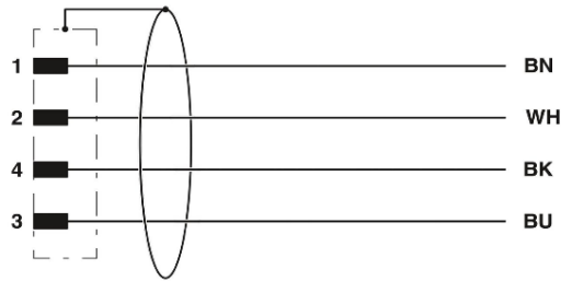
Pin assignment from M12-plug
