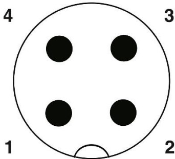
Pin assignment M12-plug, 4-pol, A-coding
