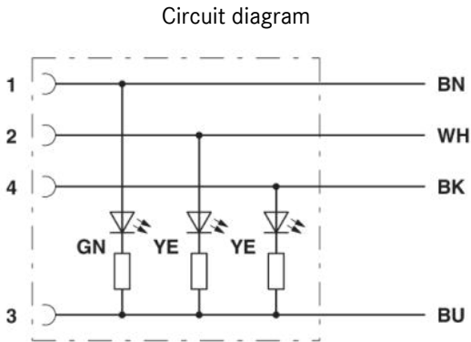
Pin assignment between M12-plug and M12-jack, with LED
