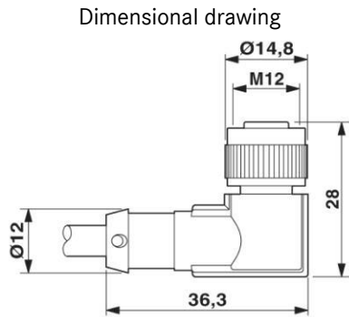
Jack M12 x 1, angled, with LED
