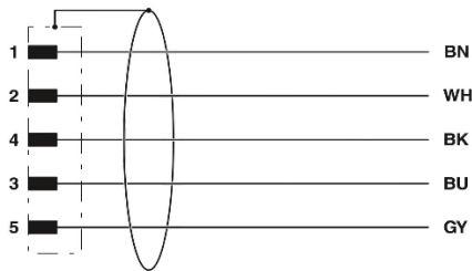
Pin assignment from M12-plug
