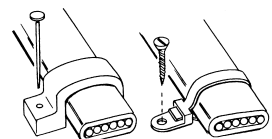
Securing cable
