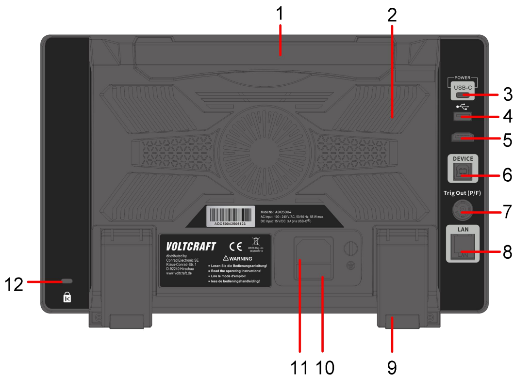
Figure 3-2: Rear Panel
