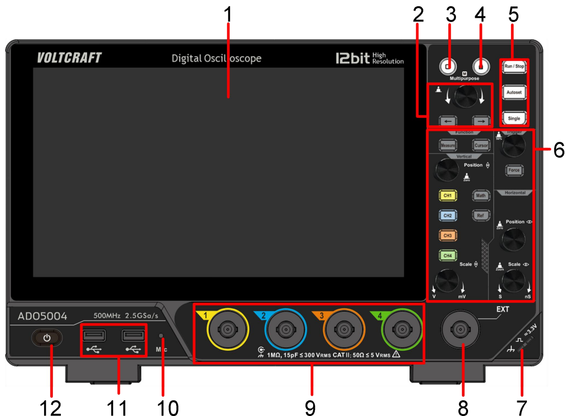
Figure 3-1: Front panel
