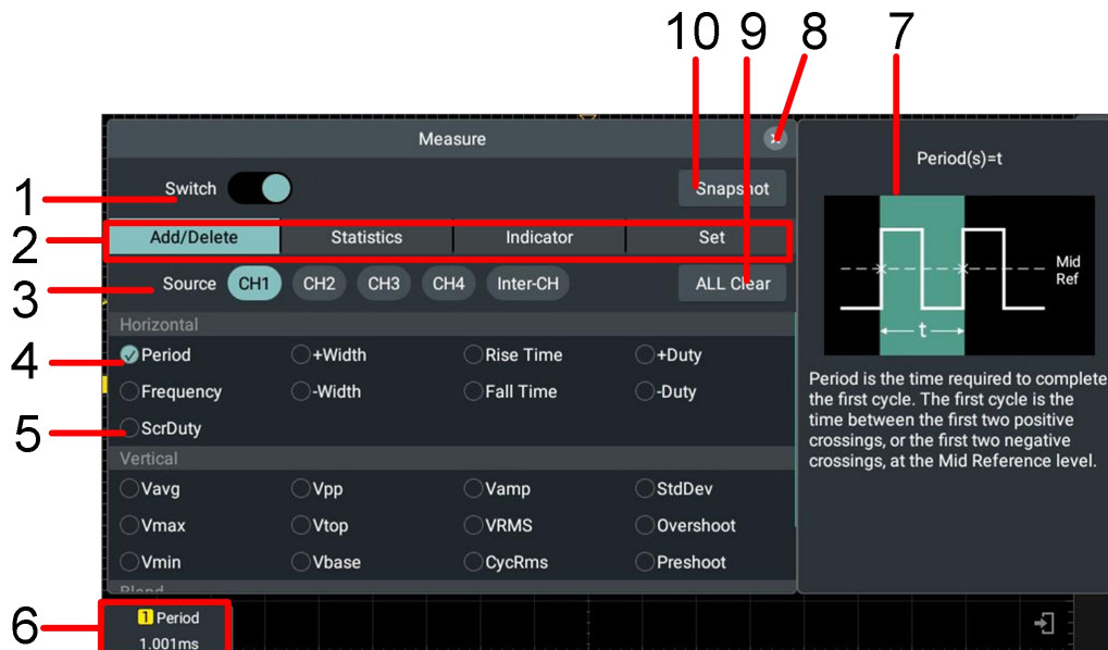
Figure 5-5: Automatic measurement
