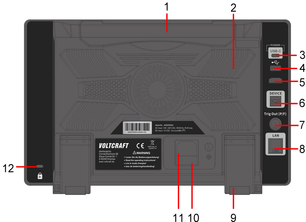
Figure 3-2: Rear Panel
