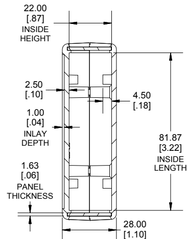
SECTION B-B SIDE VIEW
