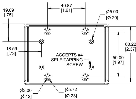
INSIDE BOTTOM
