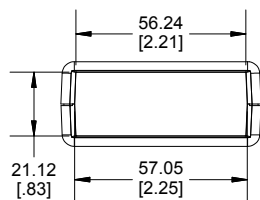
END VIEW
