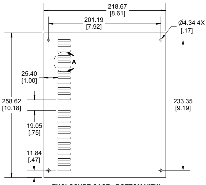
ENCLOSURE CASE - BOTTOM VIEW
