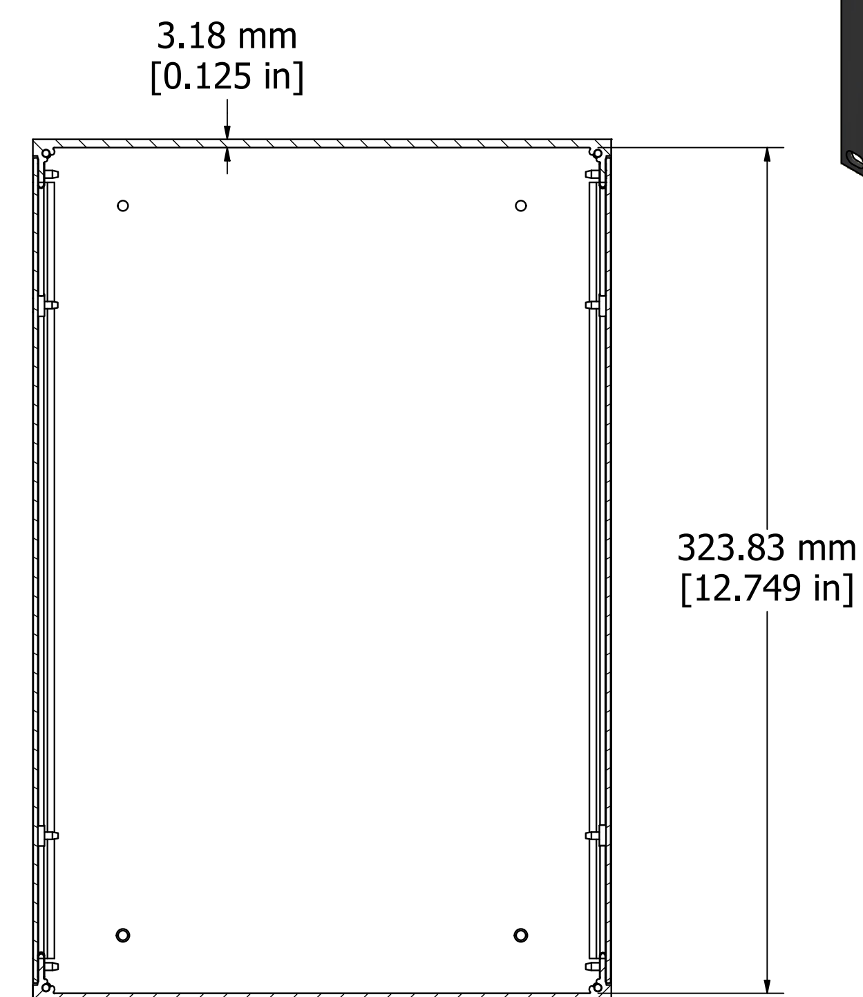
SECTION B-B
