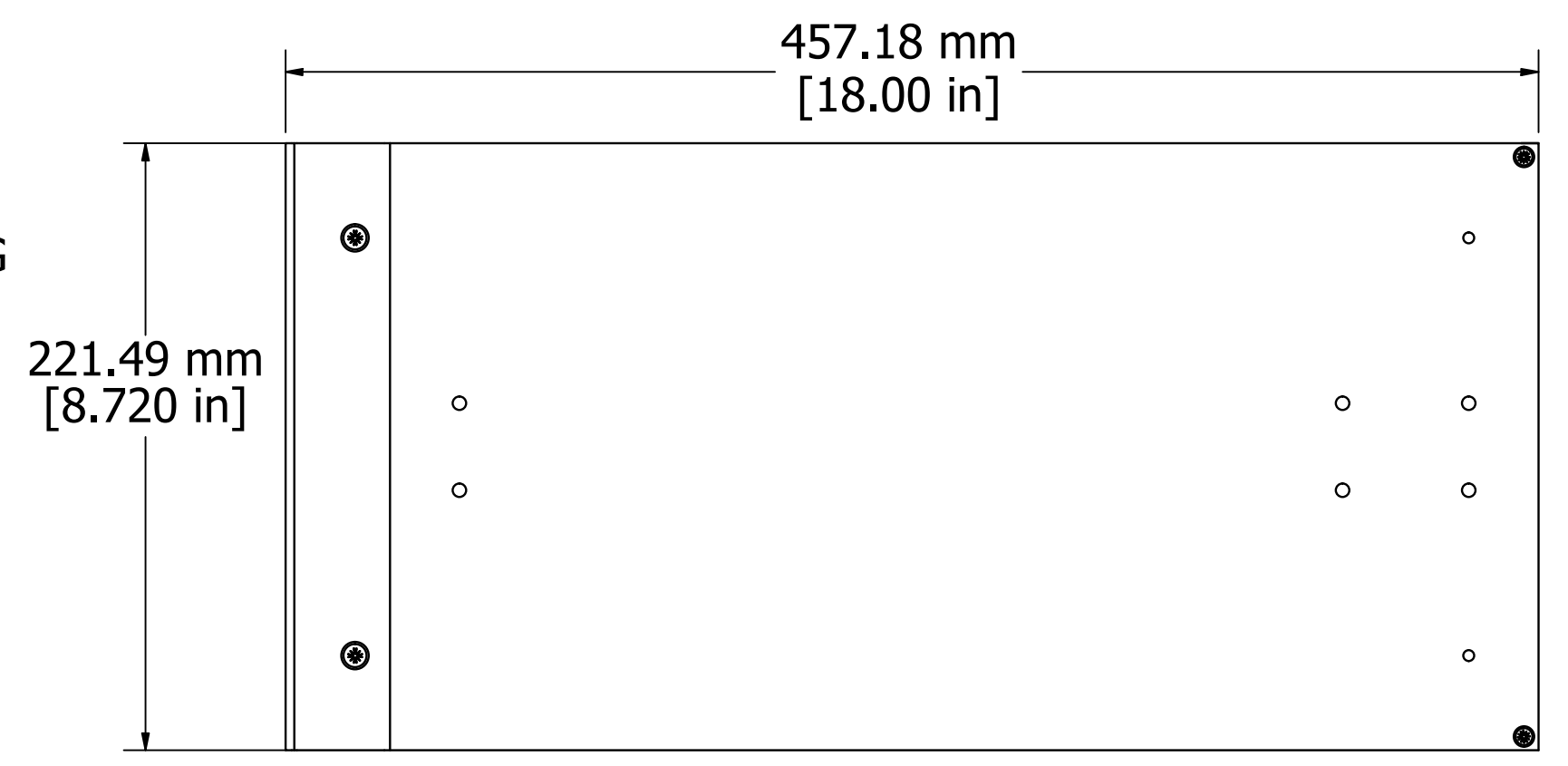
ASSEMBLY - VIEW FROM SIDE
