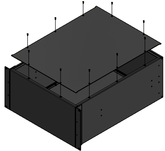
ASSEMBLY - ISOMETRIC VIEW
