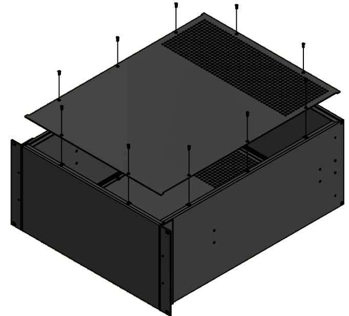
ASSEMBLY - ISOMETRIC VIEW
