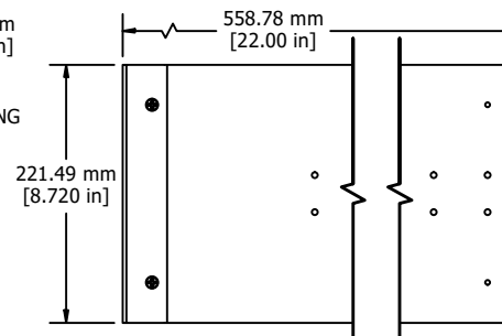
ASSEMBLY - SIDE VIEW
