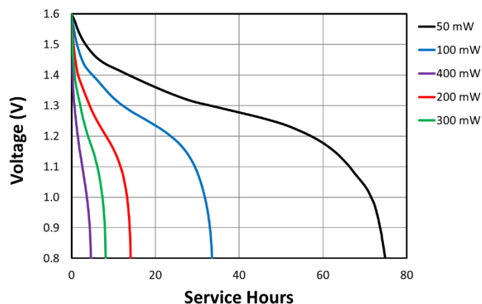
Constant Power
